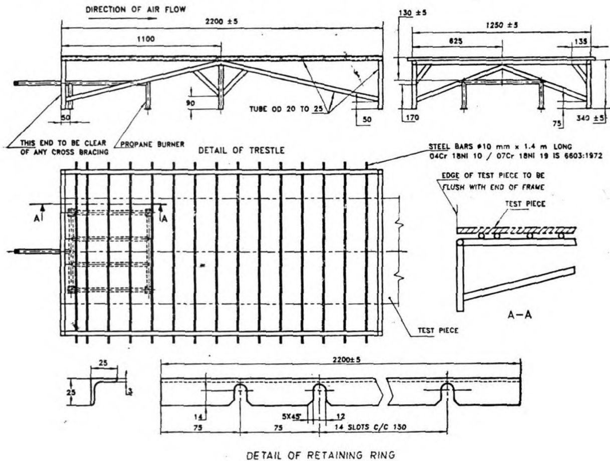
FIG. 20 PROPANE BURNER TRESTLE SHOWING POSITIONS OF BURNER AND TEST PIECE
