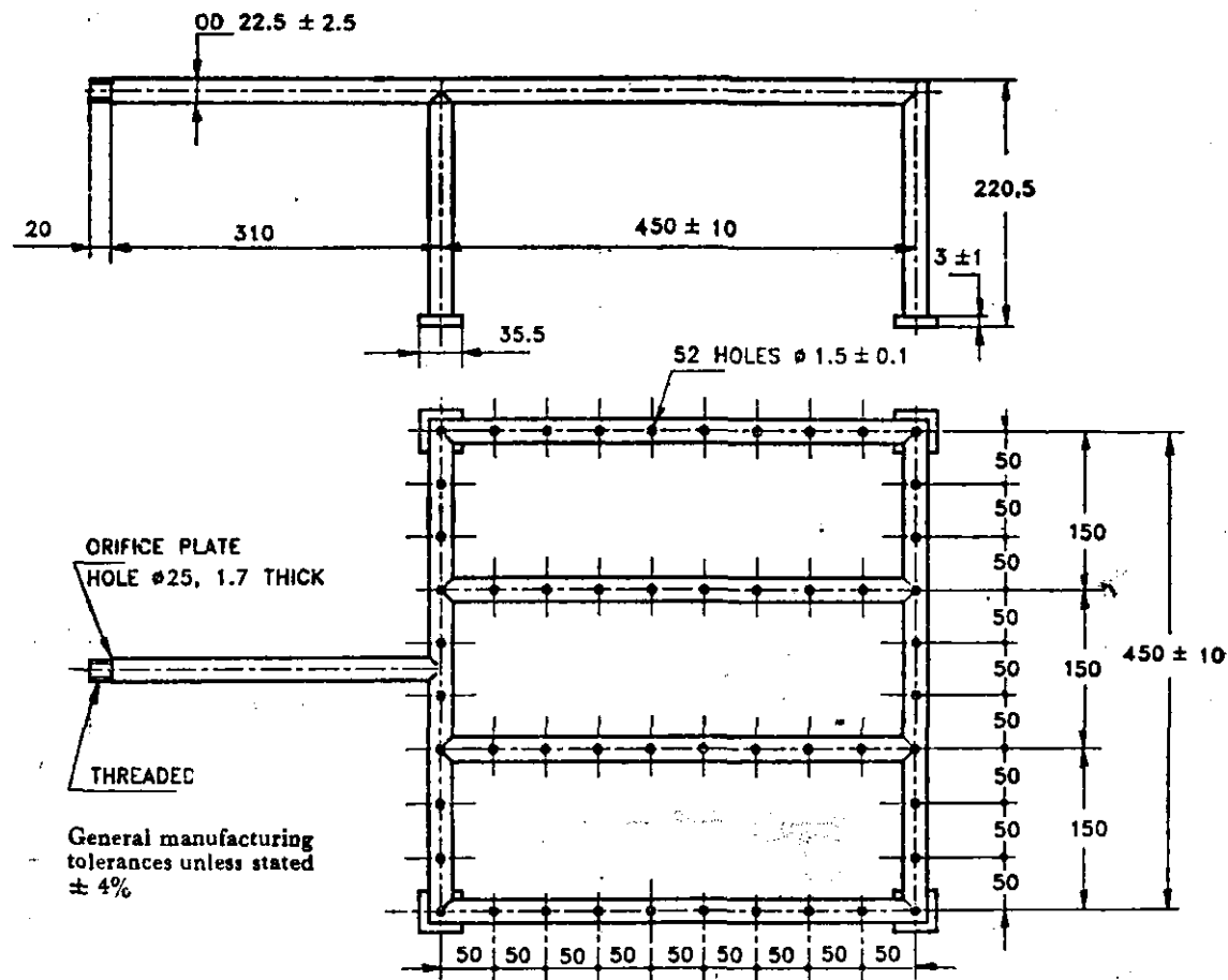
FIG. 21 PROPANE BURNER
