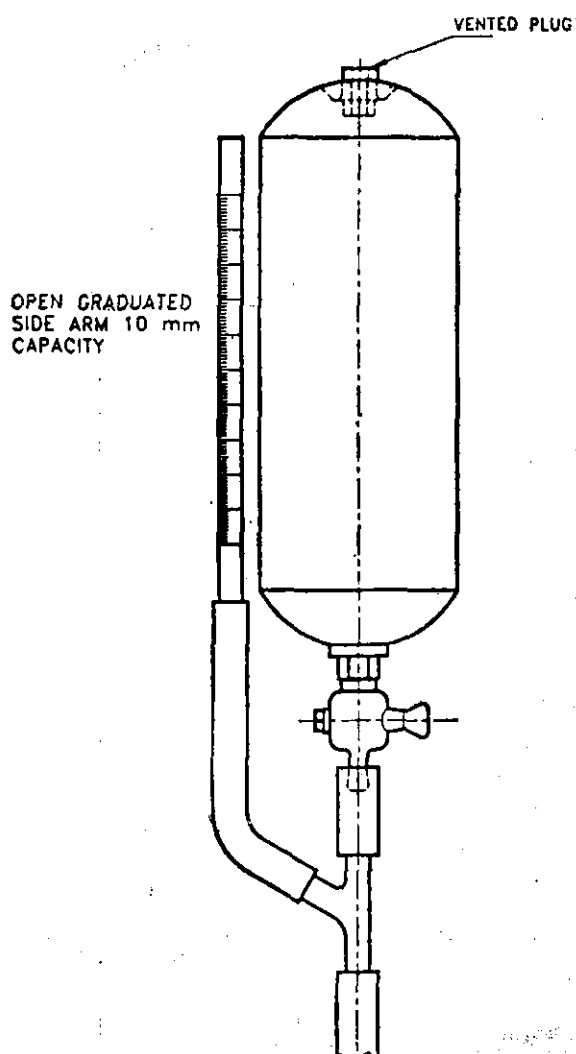
FIG. 16 RESERVOIR SIDE ARM
