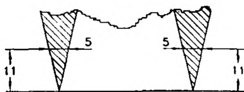
All dimensions in millimetres. FIG. 5 CROSS SECTION OF DIE
