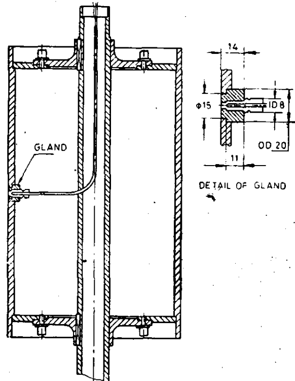
FIG. 13 ARRANGEMENT OF DRUM TEMPERATURE MEASURING DEVICE
