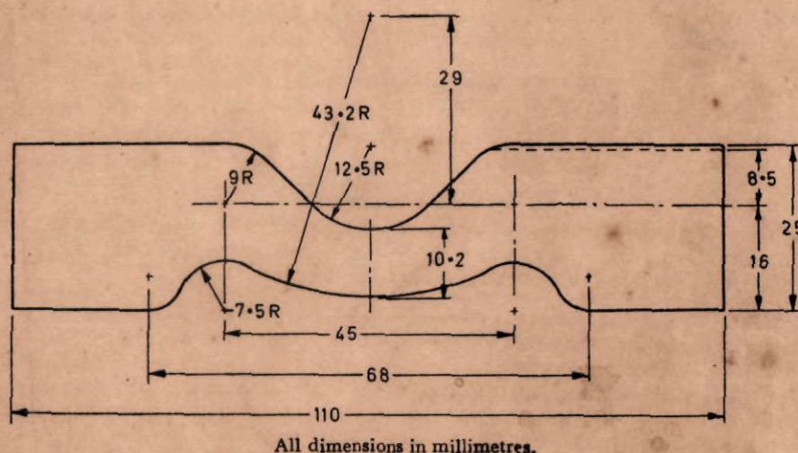
FIG. 1 CRESCENT TEST PIECES
