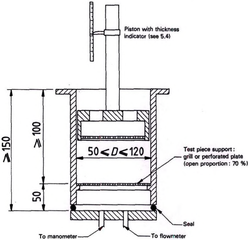
Figure 3 — Measurement cell (cylindrical section)
