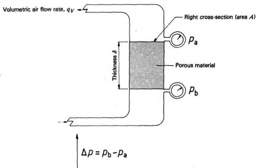
Figure 1 — Basic principle of the test (according to Darcy's laws)
