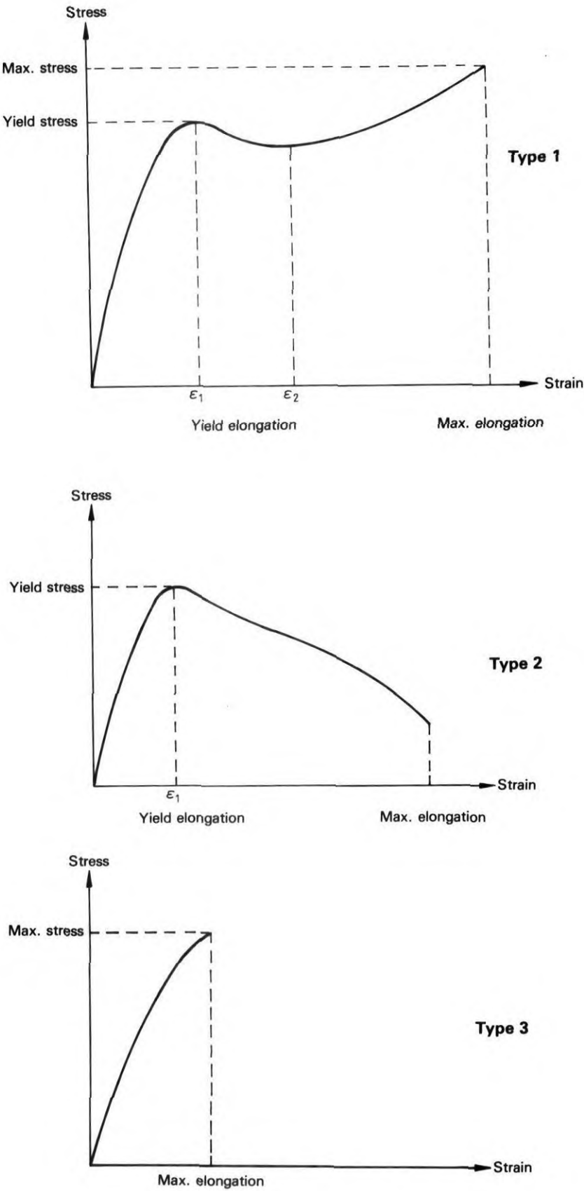
Figure 1 — Typical tensile stress-strain curves
