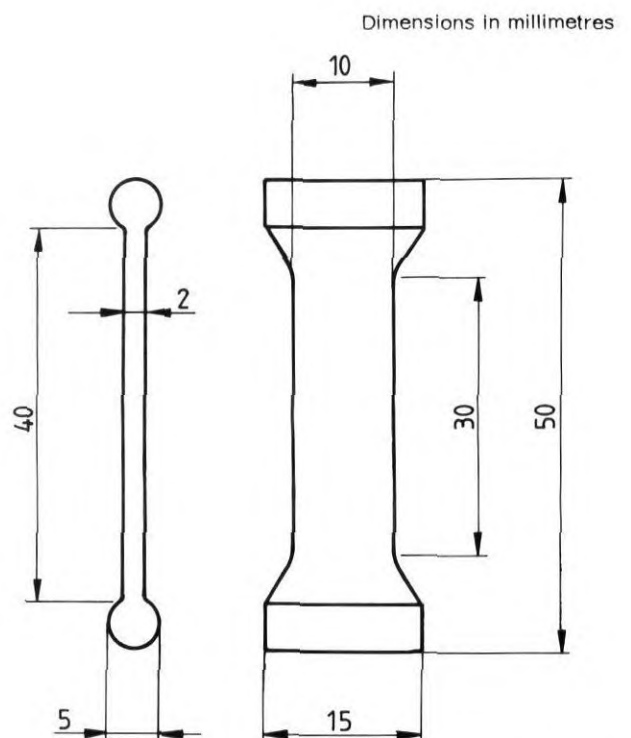
Figure 4 — Dumb-bell test piece with beaded ends
