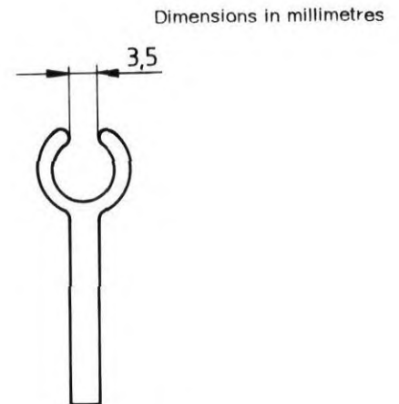
Figure 3 — Fixture with slot
