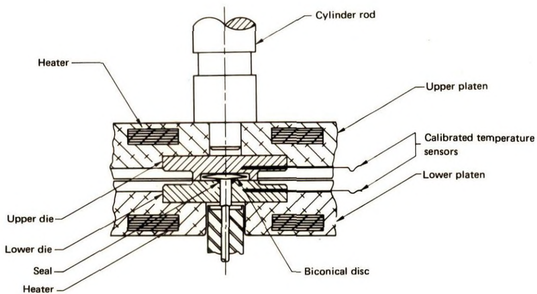
FIGURE 2 – Curemeter assembly
