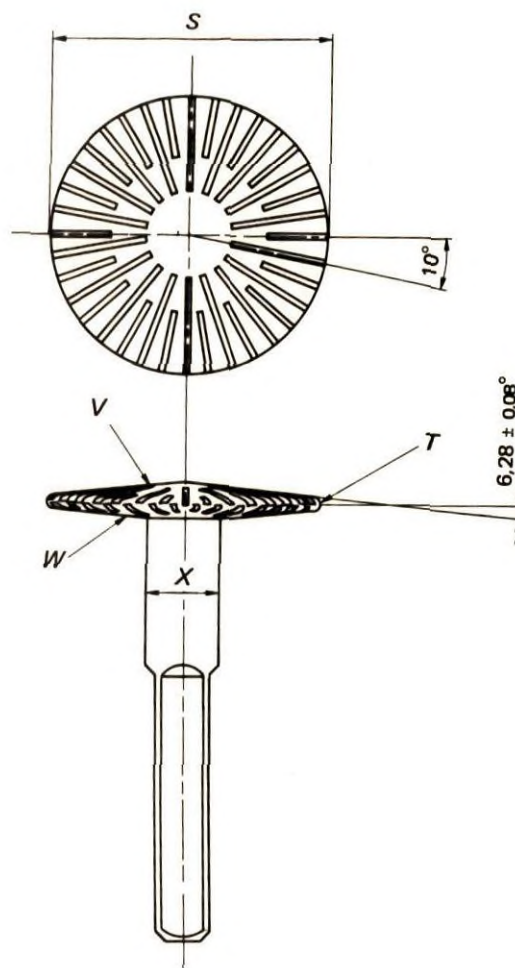
FIGURE 5 — Biconical disc
