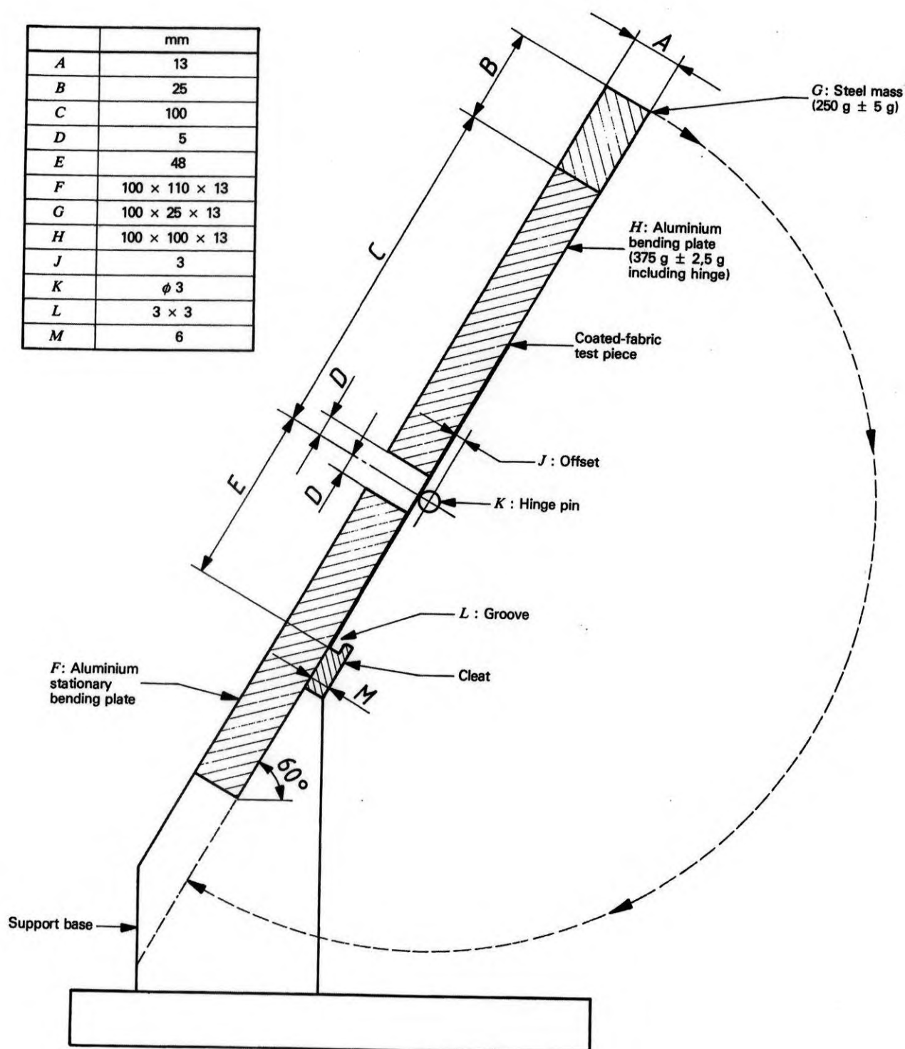
Figure 2 — Dimensions of bending jig
