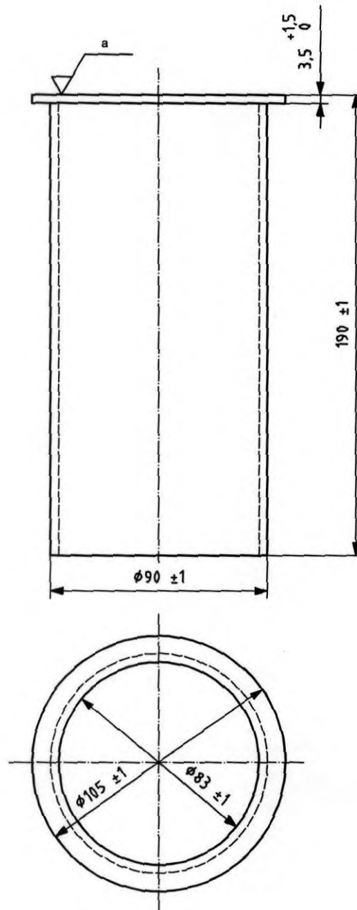
Figure 1 — Glass beaker
