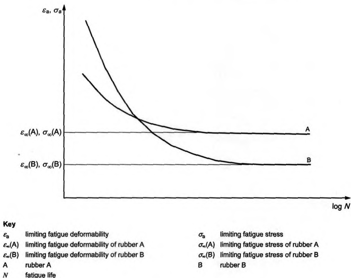
Figure 1 — Fatigue life curves for two rubbers, A and B
