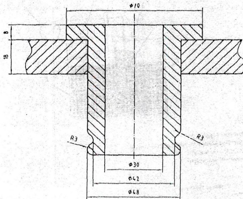
Figure L.3 — Examples of means of attaching the condom to the support
