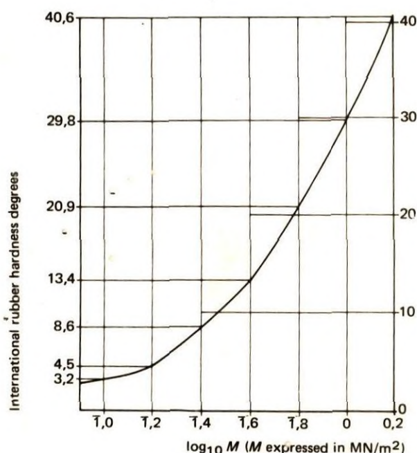
FIGURE 2 — Relation of \log_{10} M to hardness in international rubber hardness degrees
