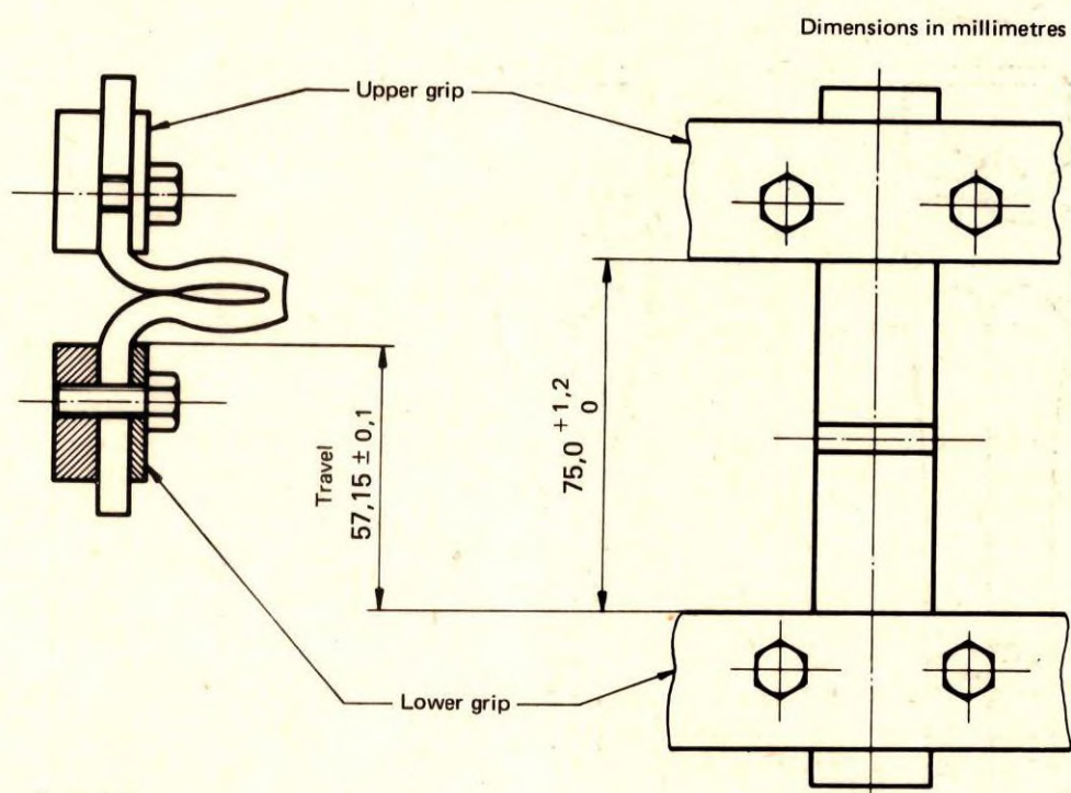
FIGURE 1 — De Mattia-type machine
