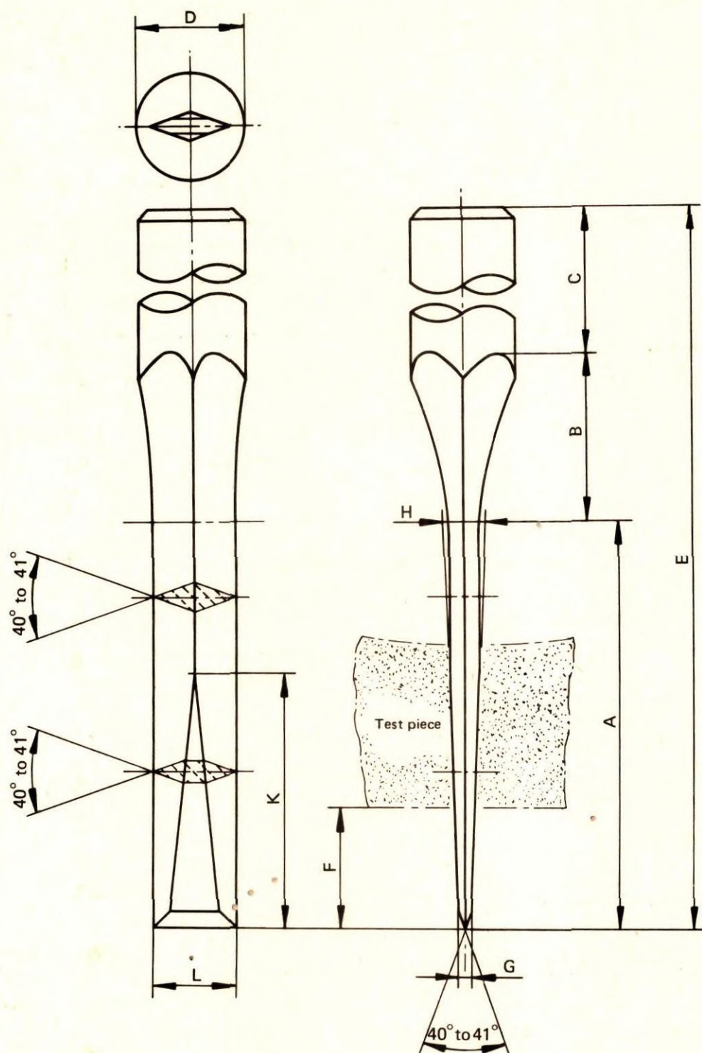
FIGURE 3 — Piercing tool
