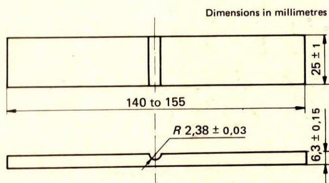
FIGURE 2 — Test piece
