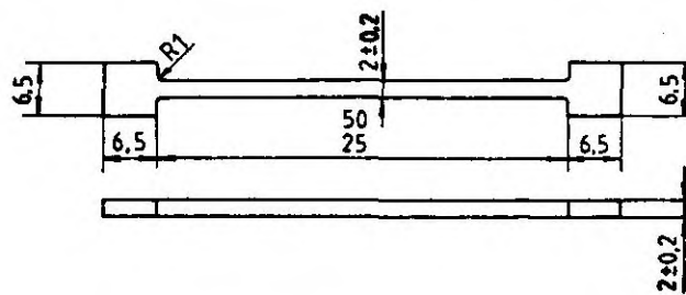
Figure 1 — Test piece with enlarged ends
