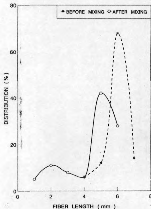
Figure 2 Fiber length distribution curve of fibers before and after mixing.
