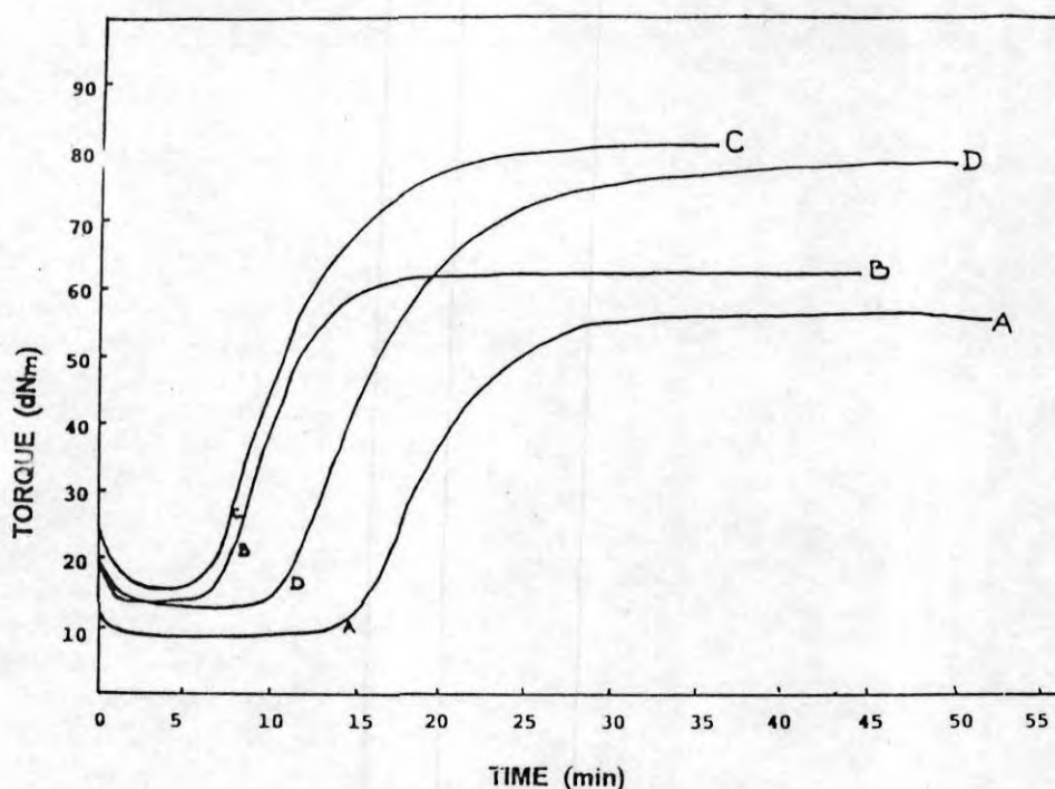
Figure 3 Rheographs of mixes A, B, C, and D.
