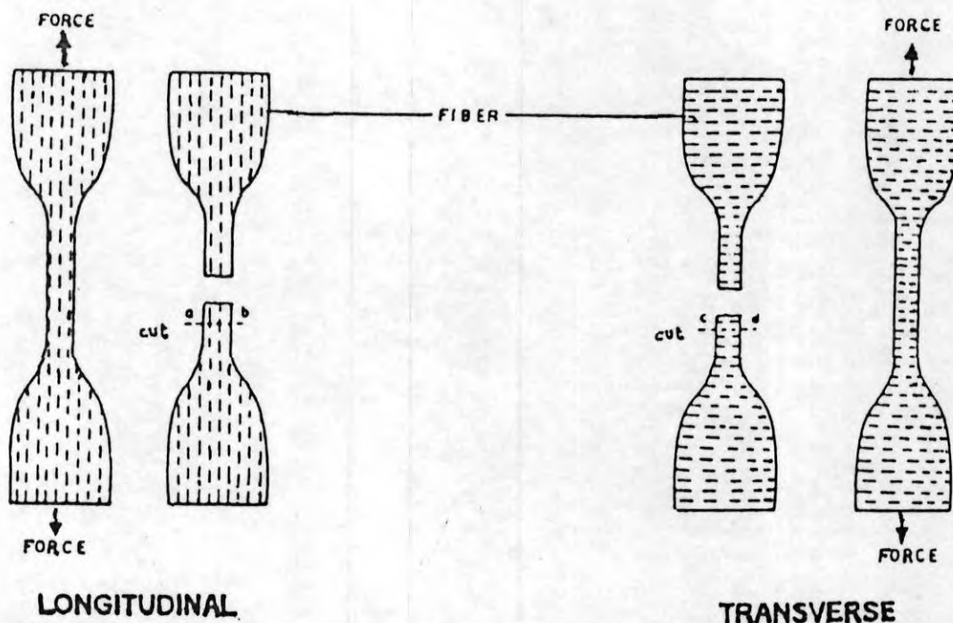
Figure 1 Tensile samples with fiber orientation and corresponding fractured surfaces.
