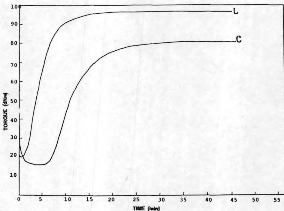
Figure 9 Rheographs of mixes C and L.
