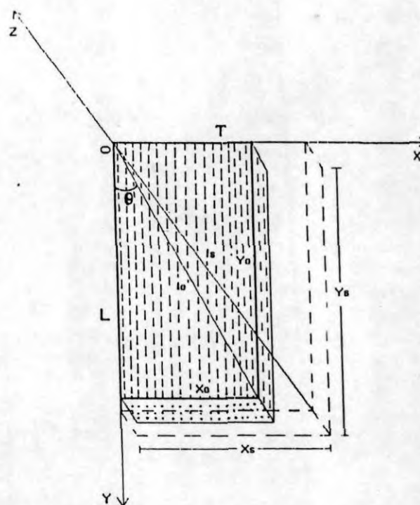
Figure 13 Geometry of the swelling of unidirectional composite.
