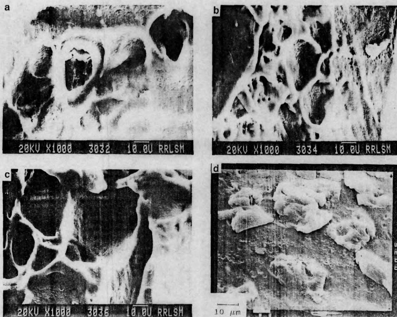
Figure 5 (a) Photomicrograph of blend G. (b) Photomicrograph of blend F. (c) Photomicrograph of blend E. (d) Photomicrograph of blend D
