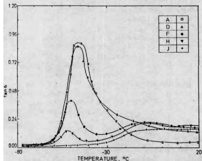
Figure 6 Effect of temperature on the loss tangent of uncrosslinked NR-EVA blends
