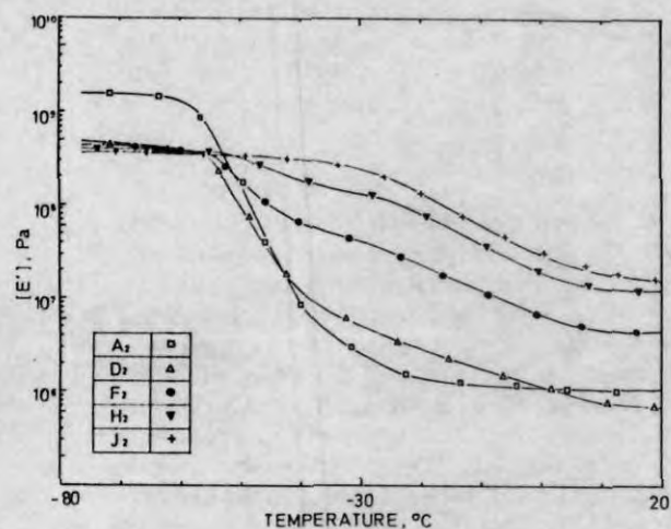
Figure 13 Effect of temperature on the storage modulus of peroxide-cured NR-EVA blends
