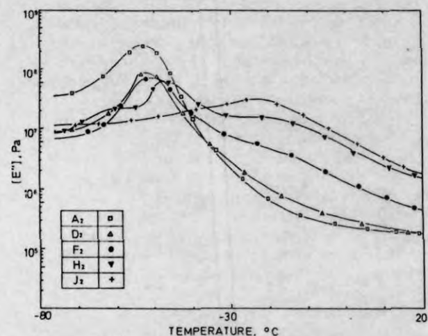
Figure 14 Effect of temperature on the loss modulus of peroxide-cured NR-EVA blends
