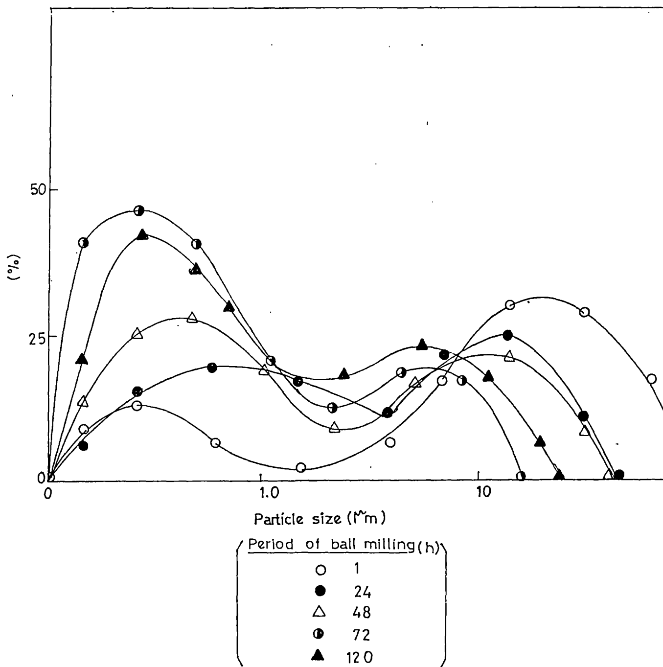
FIG.1. EFFECT OF BALL MILLING PERIOD ON PARTICLE SIZE
